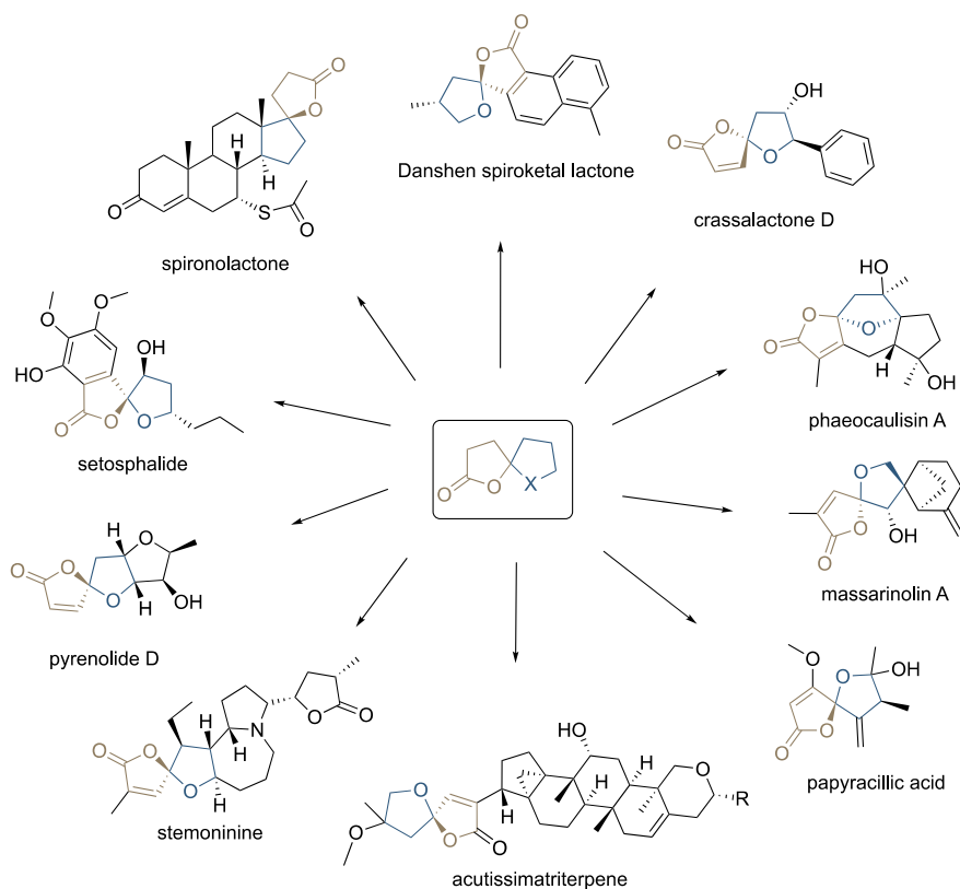
Figure 1. Biologically active spiro lactone metabolites.
