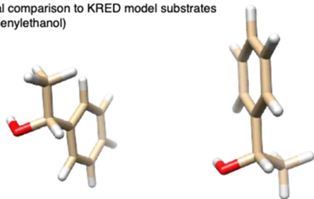
Figure 2. Configurational and geometrical analysis: (a) thermodynamic analysis of spirocyclic hemiacetal diastereomers and (b) comparison with (S)- and (R)-phenylethanol as the model substrate for the optimization of typical commercial KRED biocatalysts.
