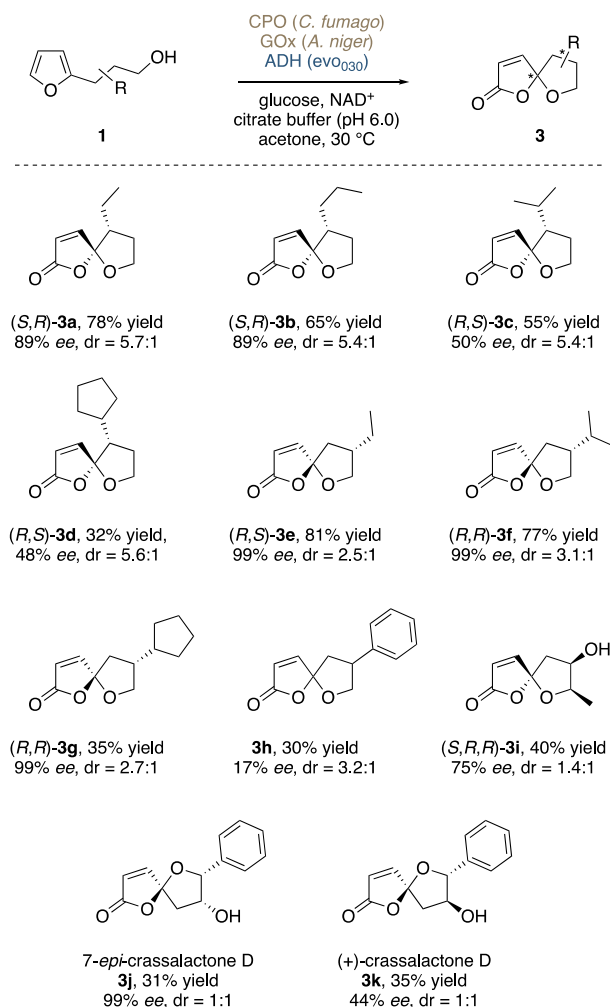
Scheme 5. Substrate Scope of the Triple-Enzymatic System for the Conversion of 3-Furylpropanols to Spirolactones a
